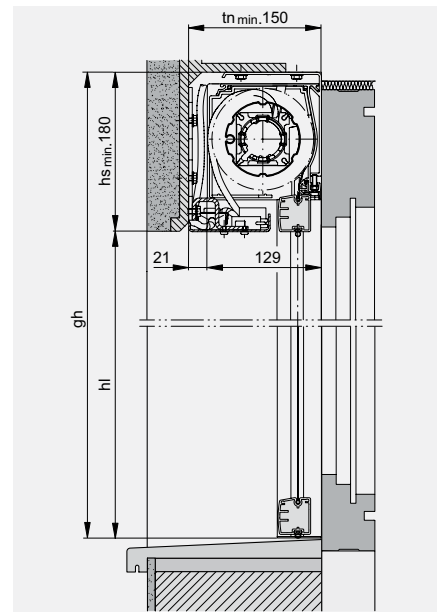
Solozip® II Box 130 angular
